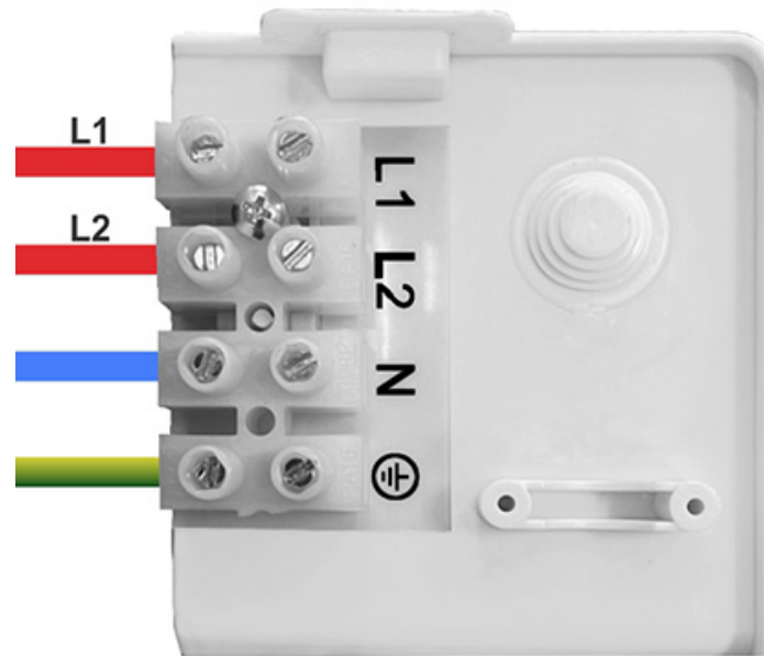
Dual-phase Connection
