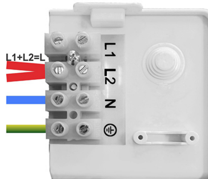
Single-phase Connection
