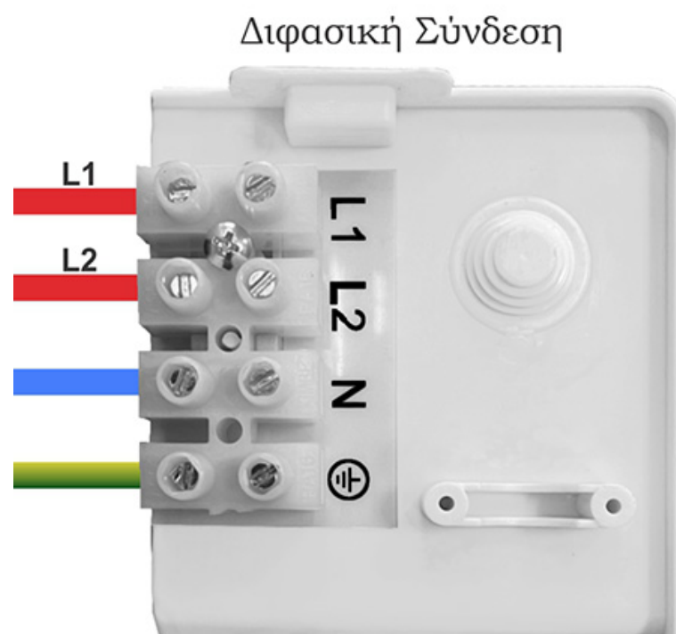
Dual-phase Connection
