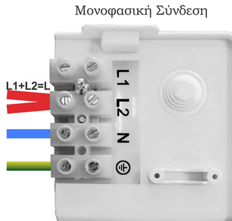
Single-phase Connection
